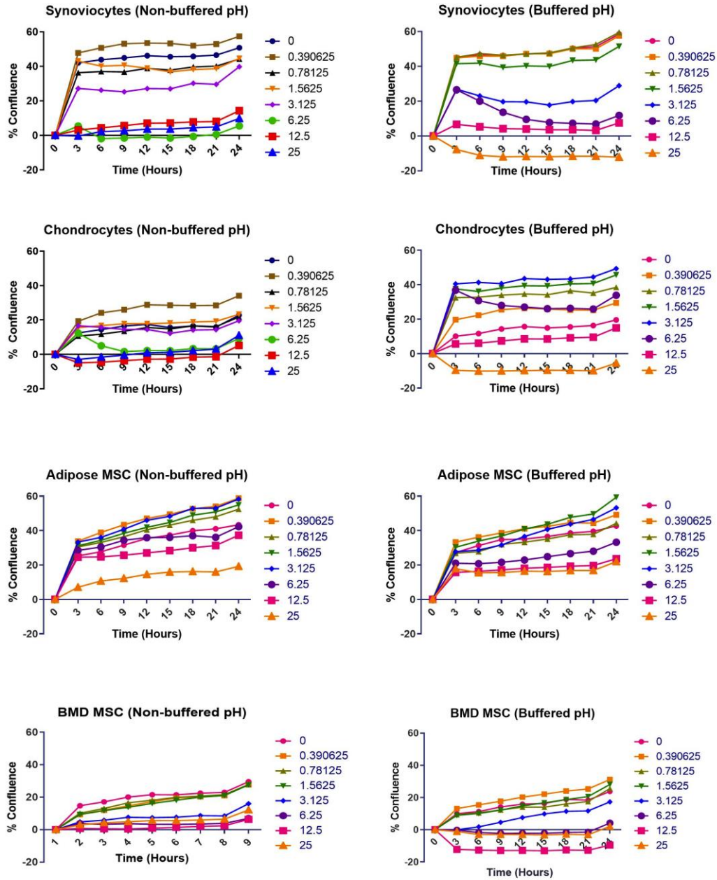
Figure 3: Effect of amikacin concentration and media pH on cell proliferation over time. When proliferation was assessed by confluence of cells over 24h using live cell imaging, there was a concentration dependent reduction in cell proliferation. At clinically relevant doses, amikacin suppressed proliferation of resident joint cells at 24h.
